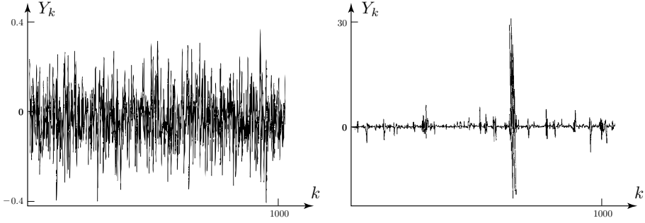
Figure 2.5: Output \mathbf{Y} of the SAC model. The sample path shown on the left was obtained using \sigma_z = 0.2 , and the one shown on the right used \sigma_z = 1.1 . In each case \alpha = 0.99 and \sigma_w = 0.1
