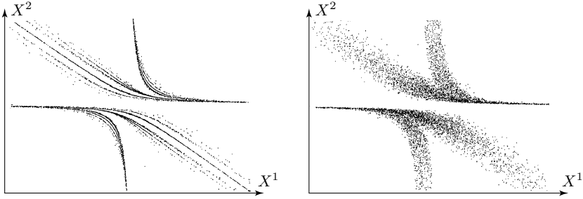
(b) Shown on the left is the gumleaf attractor, and on the right is the gumleaf attractor perturbed by noise.
