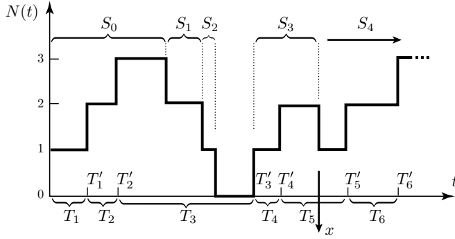
Figure 2.7: Typical sample path of the single server queue
