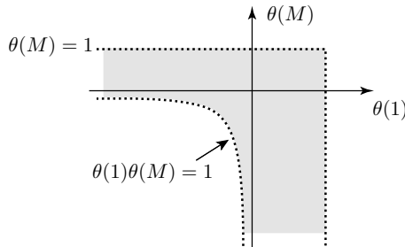
Figure B.1: The SETAR model: stability classification of (\theta(1), \theta(M)) -space. The model is regular in the shaded “interior” area (11.36), and transient in the unshaded “exterior” (9.46), (9.47) and (9.50). The boundaries are in the figures below.
