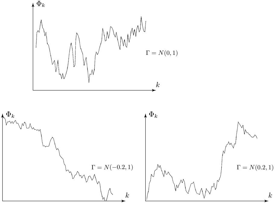
Figure 1.2: Random walk sample paths from three different models. The increment distribution is \Gamma = N(0, 1) for the path shown at top. The increment distribution is \Gamma = N(-0.2, 1) for the path shown on the lower left, and \Gamma = N(+0.2, 1) for the path shown on the lower right.
