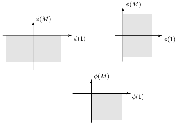
Figure B.2: The SETAR model: stability classification of (\phi(1), \phi(M)) -space in the regions (\theta(M) = 1; \theta(1) \leq 1) and (\theta(M) \leq 1; \theta(1) = 1) . The model is regular in the shaded “interior” areas, which are (clockwise starting with the plot on the far left) (11.38), (11.37) and (11.39); transient in the unshaded “exterior” (9.49), (9.48); and null recurrent on the “margins” described clockwise by (11.45), (11.46) and (11.47)–(11.48).
