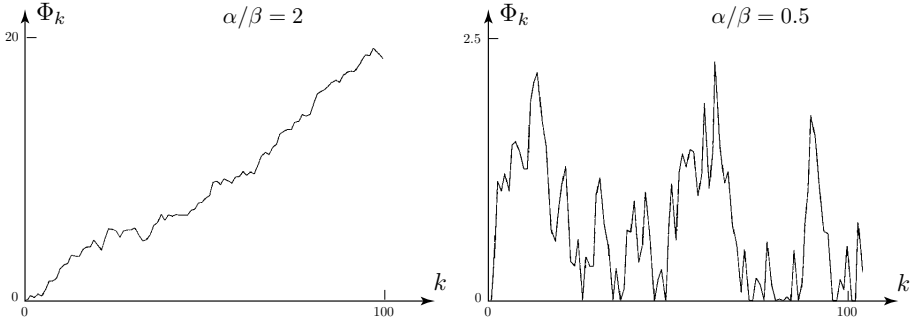
Figure 2.8: Storage system paths. The plot shown on the left uses \alpha/\beta = 2 , and on the right \alpha/\beta = 0.5 . In each case r = 1 .
