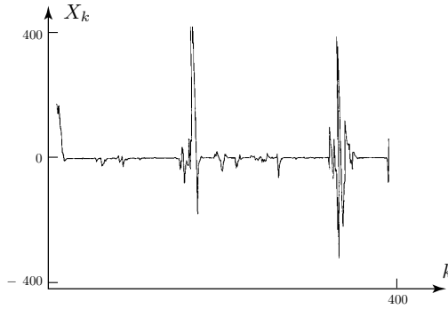
Figure 2.2: Simple bilinear model path with F(x, w) = (0.707 + w)x + w
