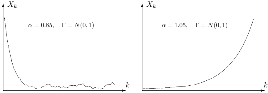
Figure 2.1: Shown on the left is a sample path from the linear model with \alpha = 0.85 , and shown on the right is a sample path obtained with \alpha = 1.05 . The increment distribution is N(0, 1) in each case.
