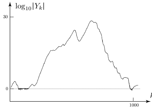
Figure 16.1: The output of the simple adaptive control model when the control U_k is set equal to zero. The resulting process is equivalent to the dependent parameter bilinear model with \alpha = 0.99 , W_k \sim N(0, 0.01) and Z_k \sim N(0, 0.04) .
