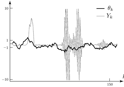
Figure 2.4: Dependent parameter bilinear model paths with \alpha = 0.933 , W_k \sim N(0, 0.14) and Z_k \sim N(0, 0.01)
