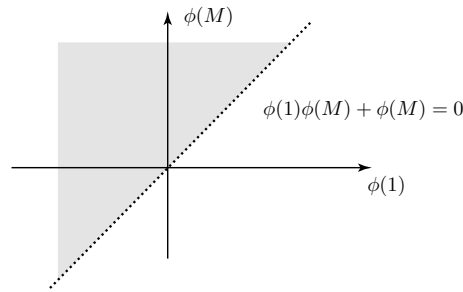
Figure B.3: The SETAR model: stability classification of (\phi(1), \phi(M)) -space in the region (\theta(M) \theta(1) = 1; \theta(1) \leq 0) . The model is regular in the shaded “interior” area (11.40); transient in the unshaded “exterior” (9.51); and null recurrent on the “margin” described by (11.49).
