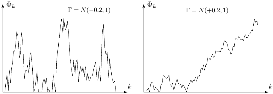
Figure 1.3: Random walk paths reflected at zero. The increment distribution is \Gamma = N(-0.2, 1) for the plot shown on the left, and \Gamma = N(+0.2, 1) for the plot shown on the right.
