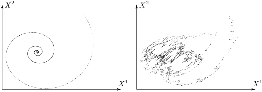
Figure 1.1: At left is a sample path generated by the deterministic linear model on \mathbb{R}^2 . At right is a sample path from the linear state space model on \mathbb{R}^2 with Gaussian noise.
