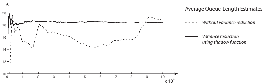
Figure 20.1: Results for a simulation run of length 100,000 steps in a network model. The dashed line represents the running average cost using the standard estimator. The solid line represents the running average cost for the estimator (20.19).
